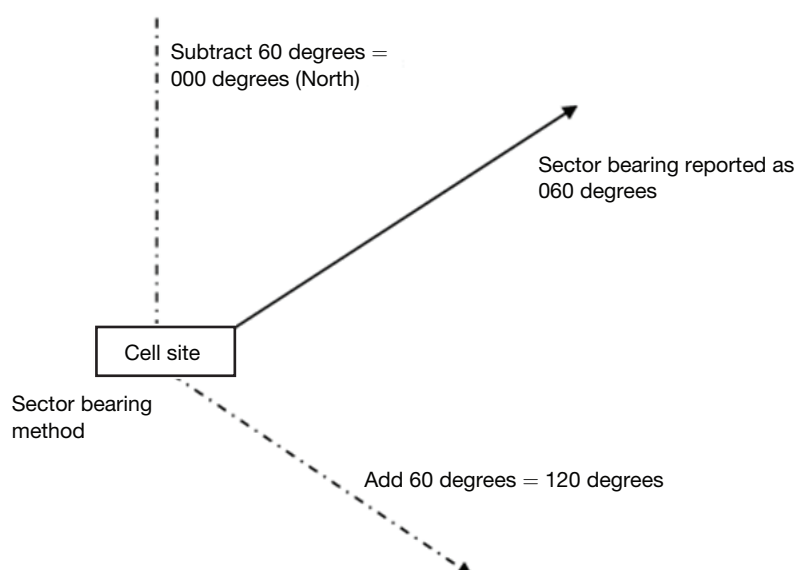
Figure U-3: Cell site sector, bearing method
