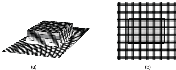
Figure 4-4 – Uniform probability density distribution with top view
