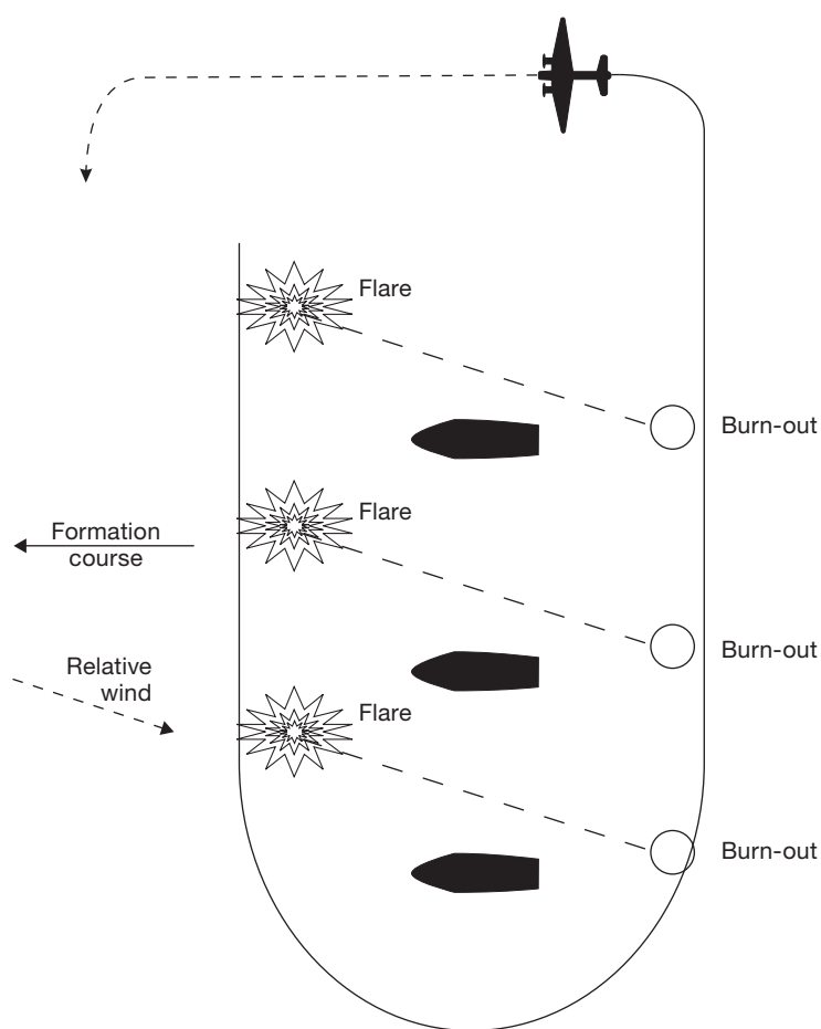
Figure 5-17 – Parachute flare search using several surface facilities
