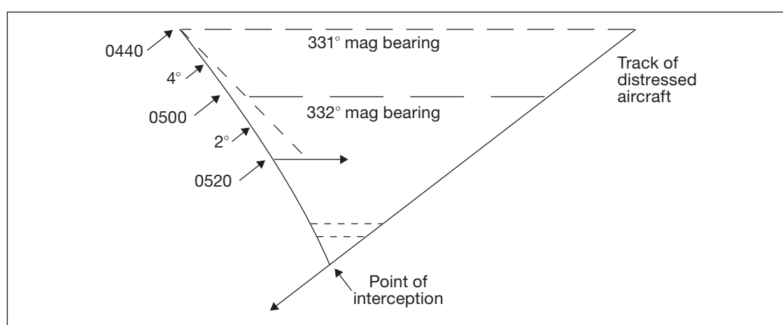
Figure J-5 – Offset or beam-on intercept: method 3
