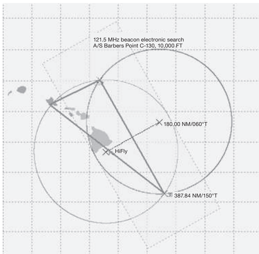
Figure S-5 – Aircraft SRU search down the intersect line at an altitude of 10,000 ft with a radio horizon range of 123 NM
