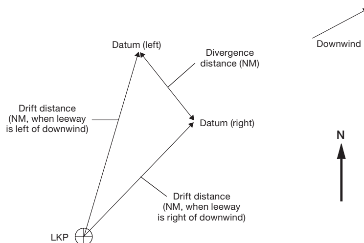
Figure 4-8 – Determining new datums and divergence distance (drift distance = drift speed × time adrift)
