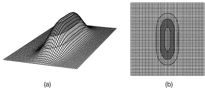
Figure 4-3 – Probability density distribution for a line datum connecting two point datums with top view
