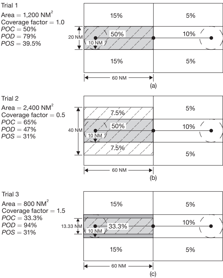
Figure 4-16 – Available effort = 1,200 NM 2
