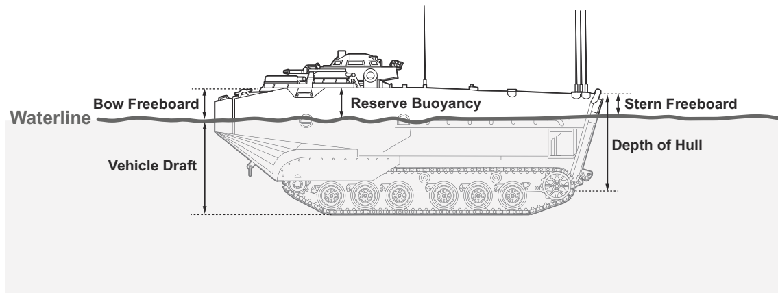
Figure 2-3. Assault Amphibious Vehicle Reserve Buoyancy.
