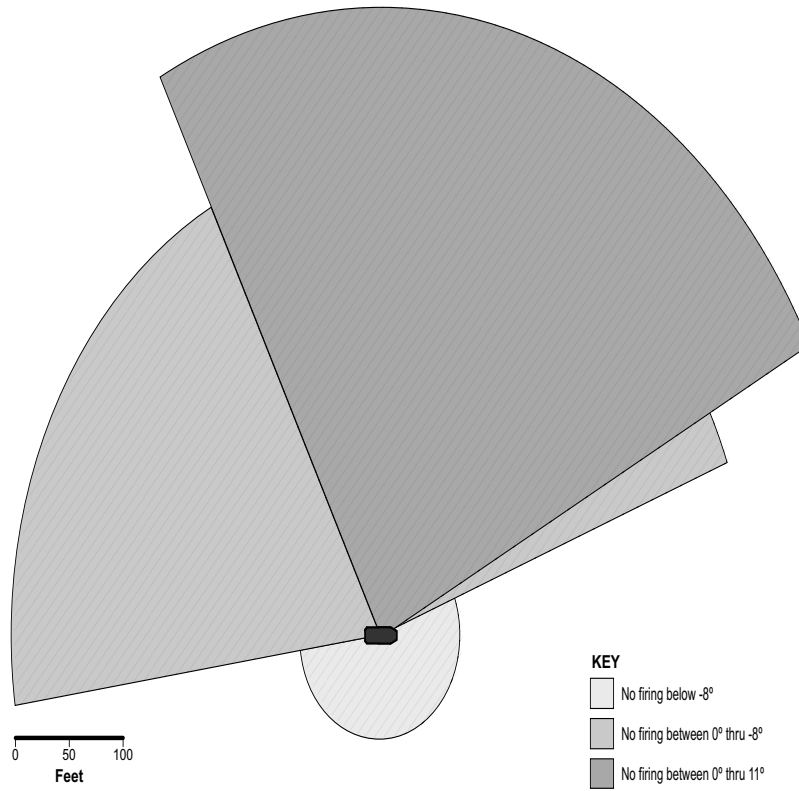
Figure 8-1. Assault Amphibious Vehicle Dead Space.
