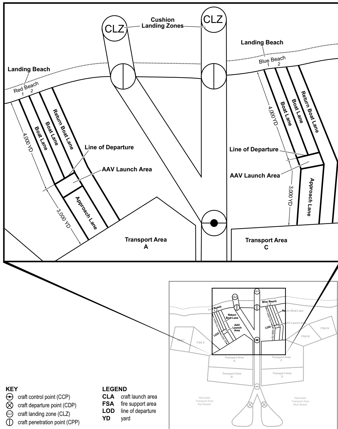
Figure 2-2. Assault Amphibious Vehicle Launching Areas.
