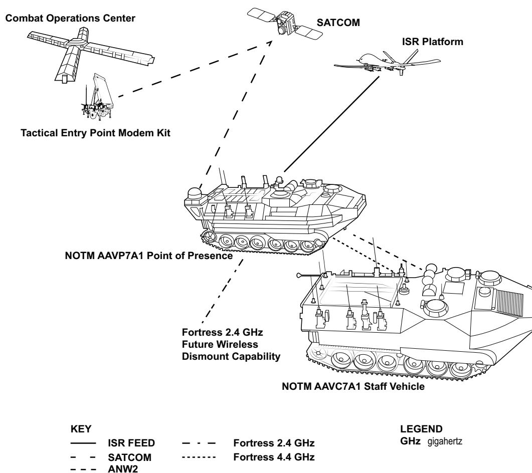
Figure 9-3. Assault Amphibious Vehicle Employment of Networking On-the-Move.
