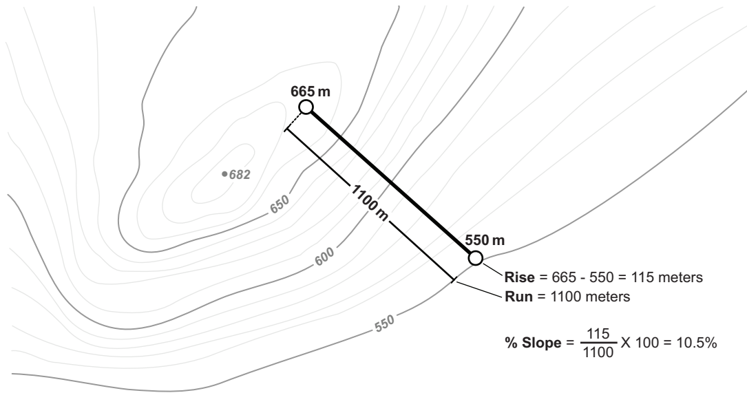
Figure A-3. Terrain Slope Calculation.
