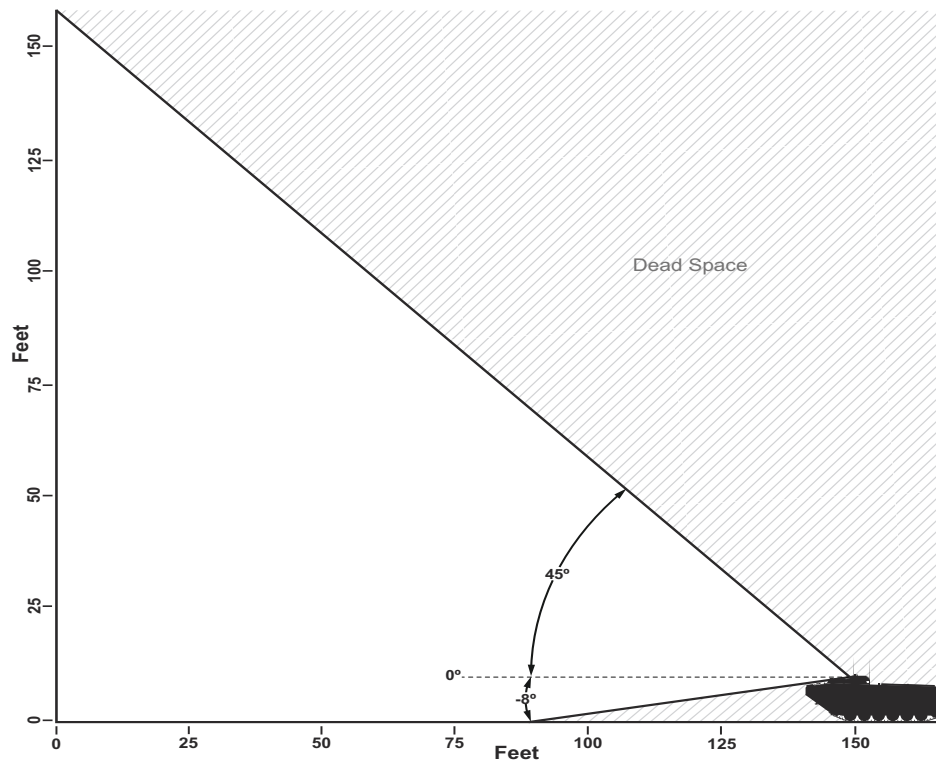
Figure 8-2. Assault Amphibious Vehicle Overhead Dead Space.
