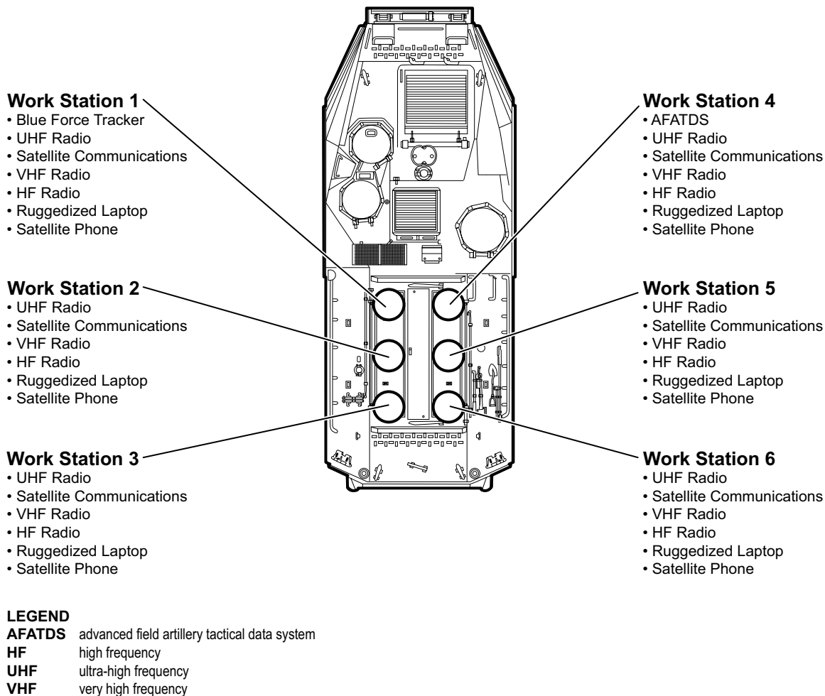
Figure 9-1. AAVC7A1 Internal Layout.
