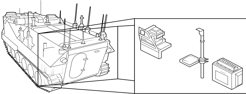
Figure B-4. AAVC7A1 with Networking On-the-Move Staff Vehicle Kit.
