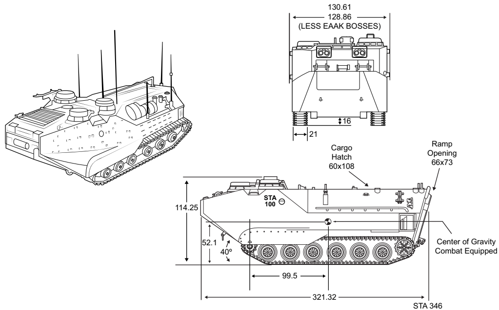
Figure B-2. AAVC7A1 Command and Control Variant Specifications.
